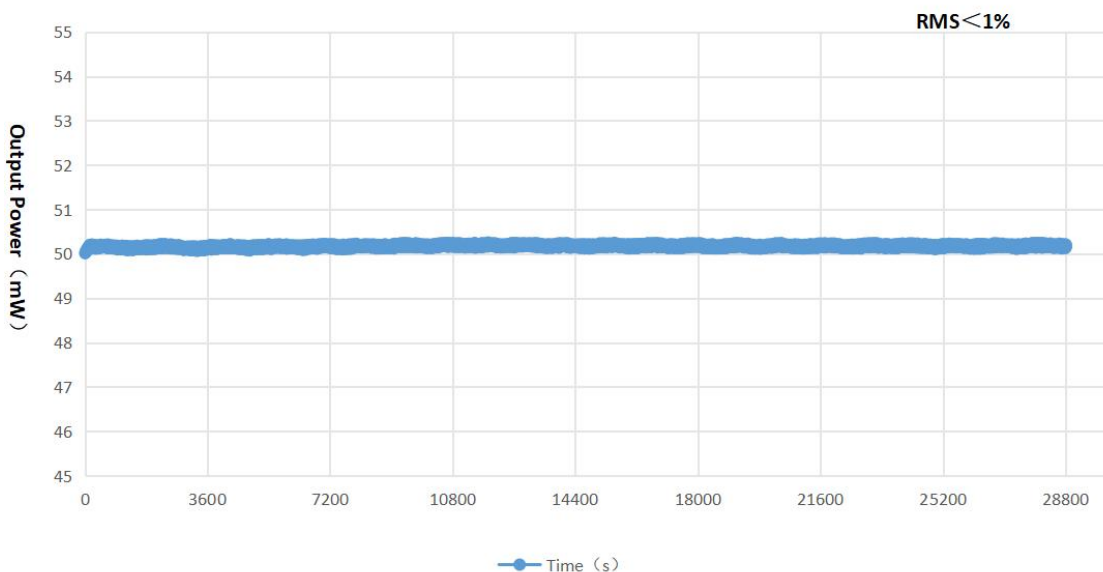
Power Stability Test 8 Hours
